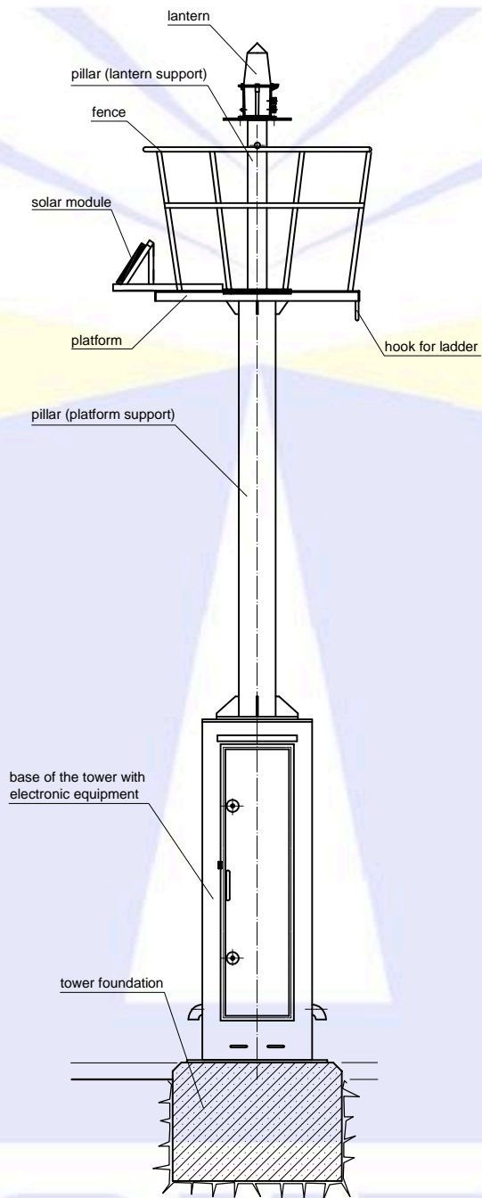
METAL TOWER TYPE "PLOVPUT 1"
